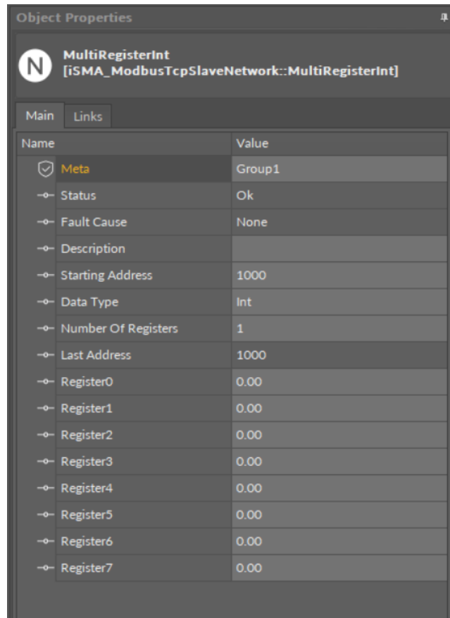
Figure 28. MultiRegisterInt component
