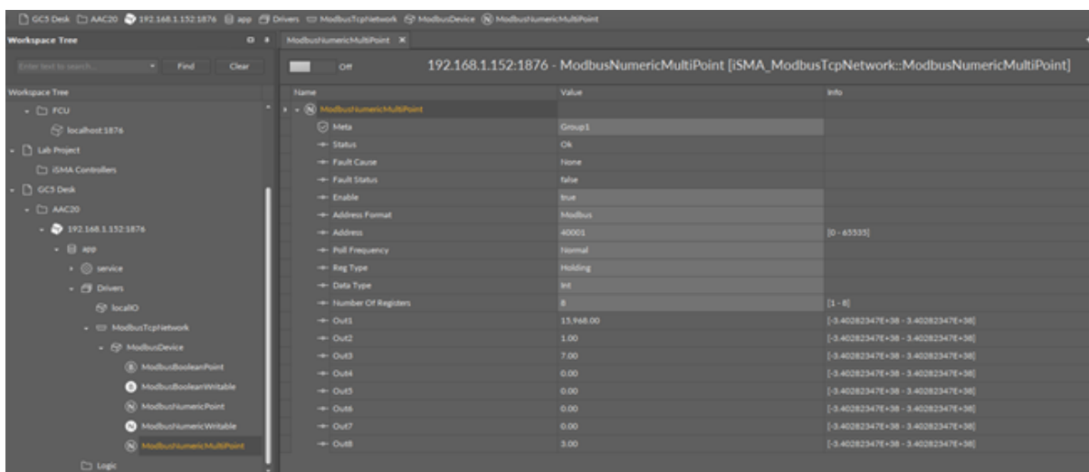
Figure 19. ModbusNumericMultiPoint
