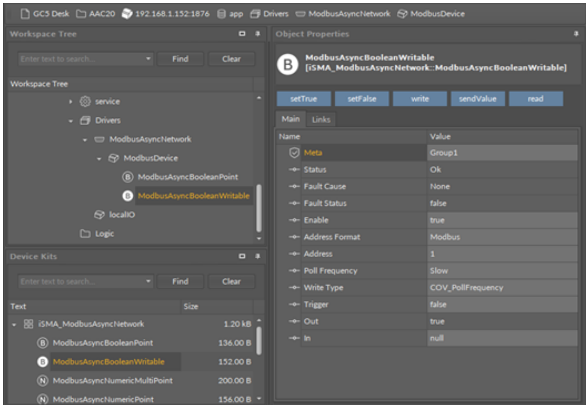
Figure 37. ModbusAsyncBooleanWritable component
