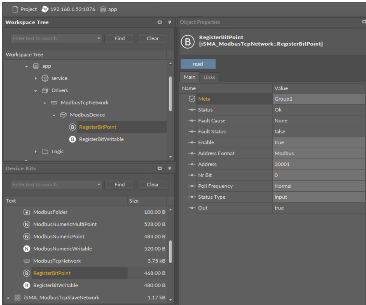
Figure 20. RegisterBitPoint
