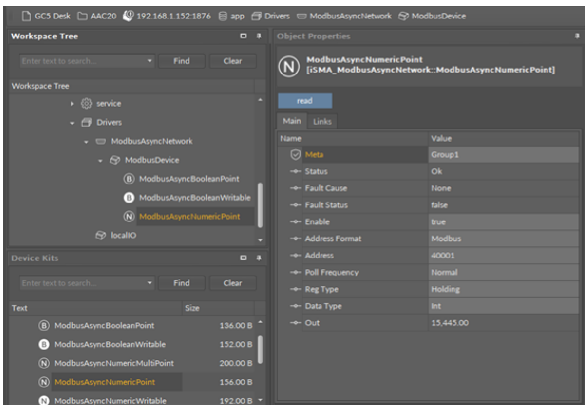
Figure 7. ModbusAsyncNumericPoint
