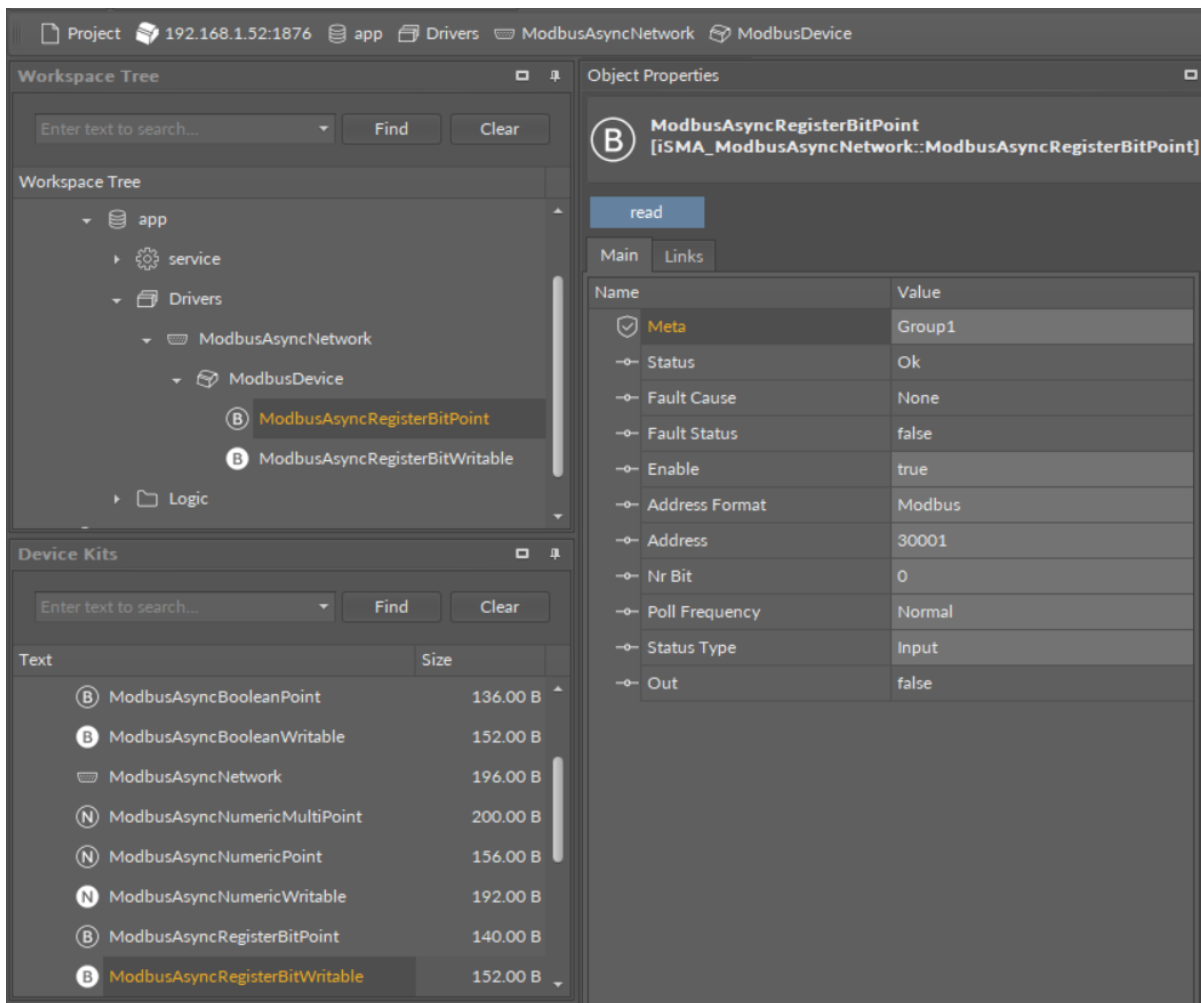
Figure 10. ModbusAsyncRegisterBitPoint component
