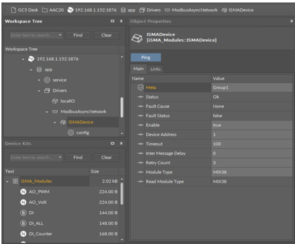
Figure 45. iSMADevice component
