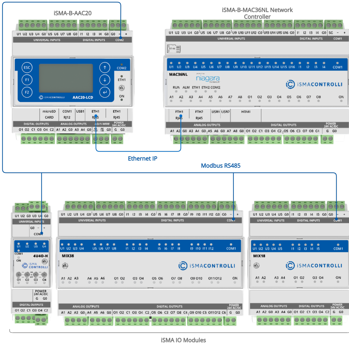
Figure 44. Modbus TCP gateway topology
