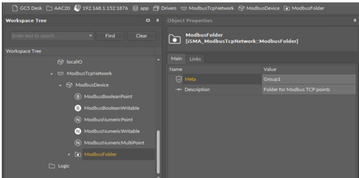
Figure 22. ModbusFolder component
