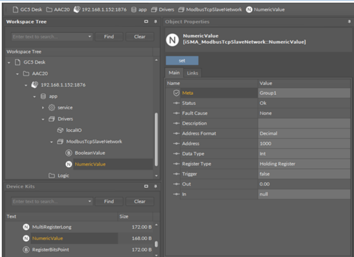
Figure 26. NumericValue component
