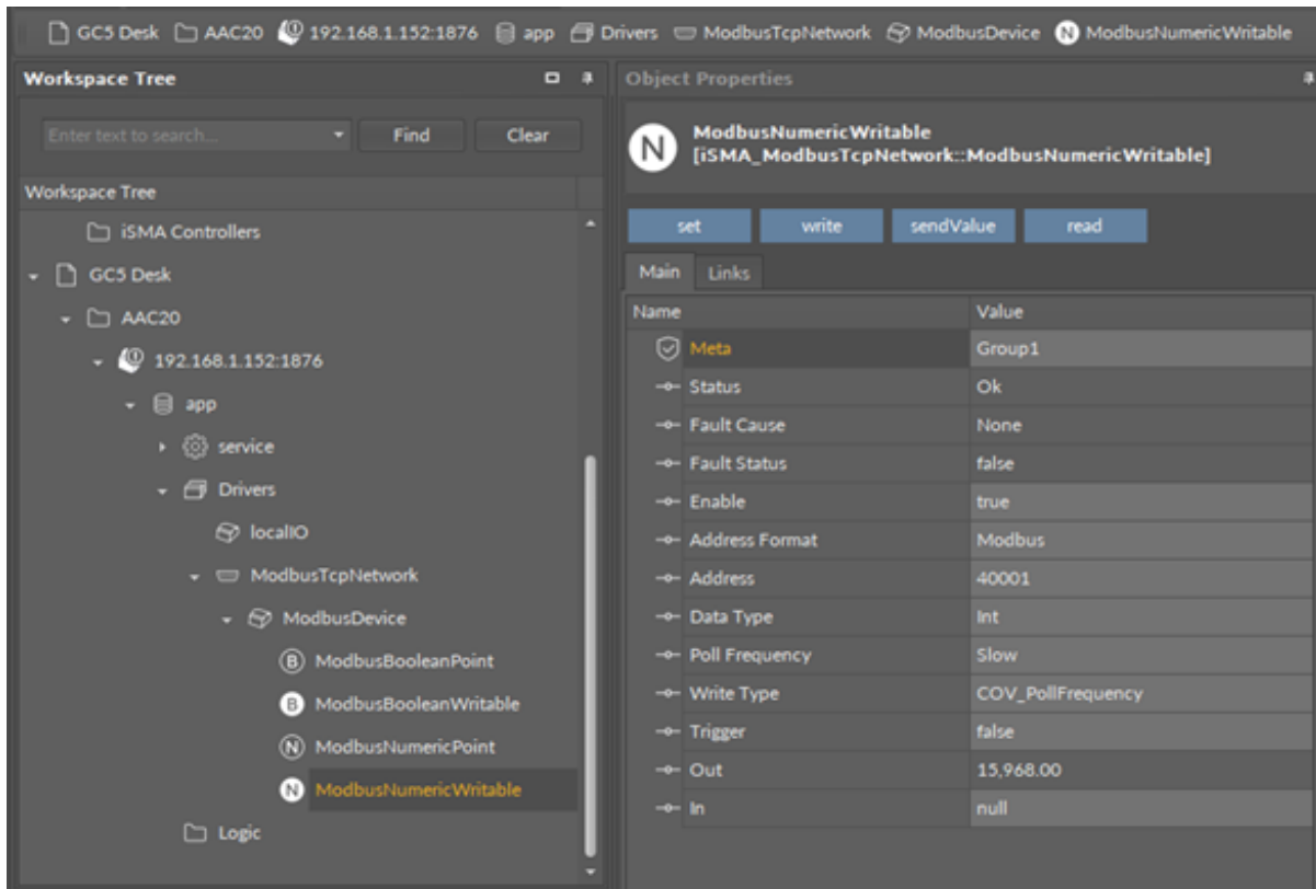
Figure 18. ModbusNumericWritable
