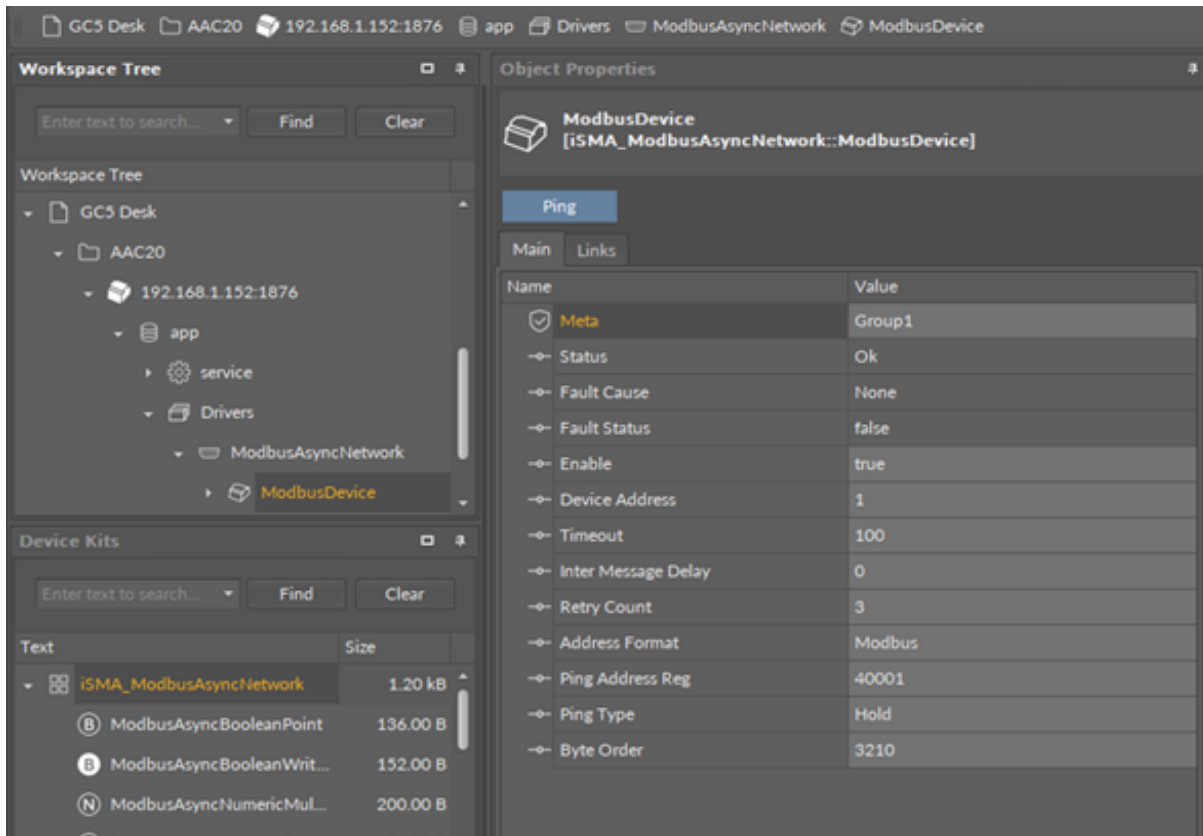
Figure 4. ModbusAsyncDevice component
