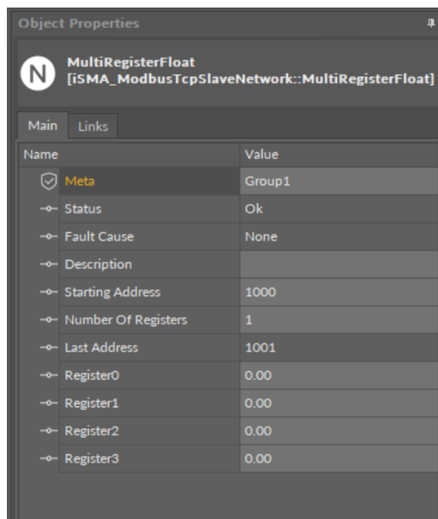
Figure 27. MultiRegisterFloat component
