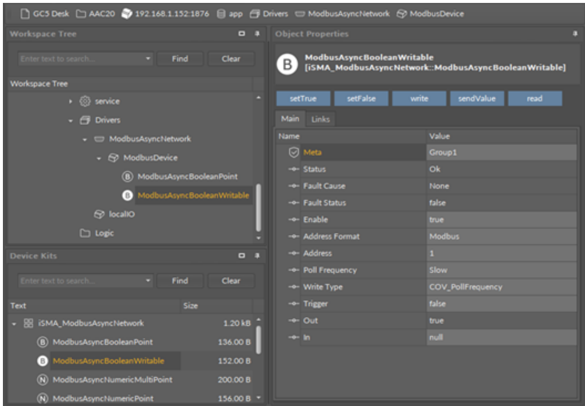
Figure 6. ModbusAsyncBooleanWritable component
