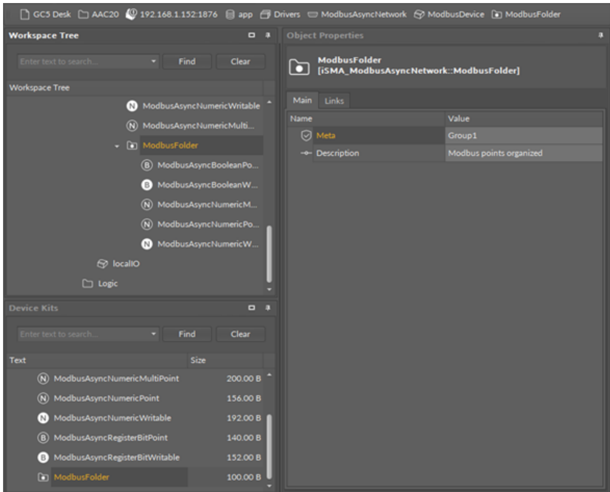
Figure 12. ModbusFolder component
