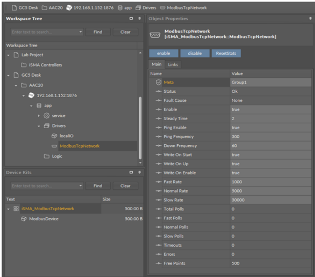
Figure 13. ModbusTCPNetwork component
