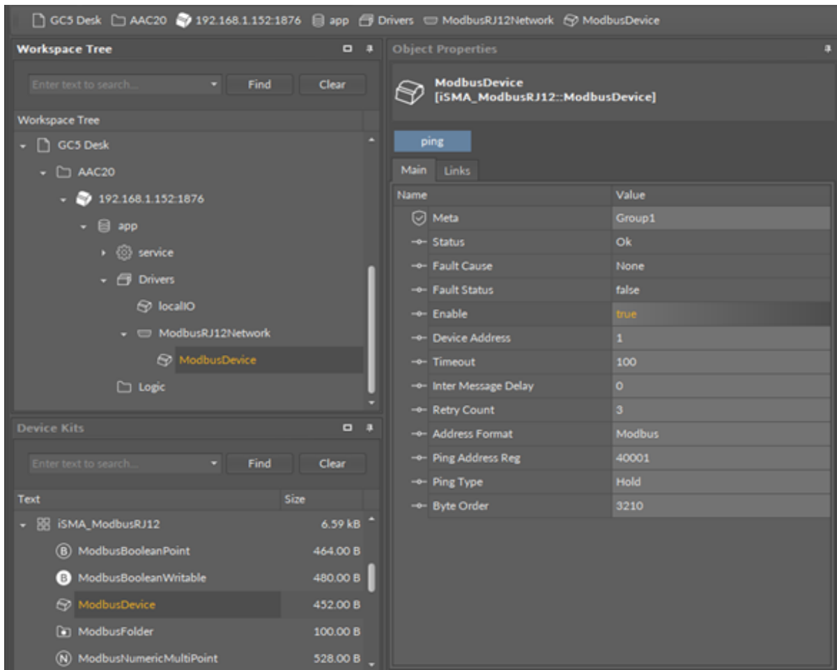
Figure 35. ModbusRJ12Device component
