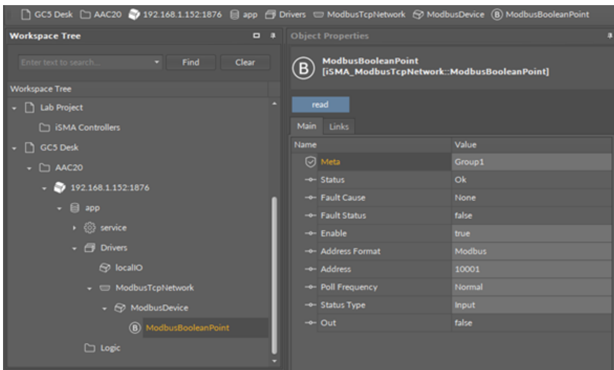
Figure 15. ModbusBooleanPoint component
