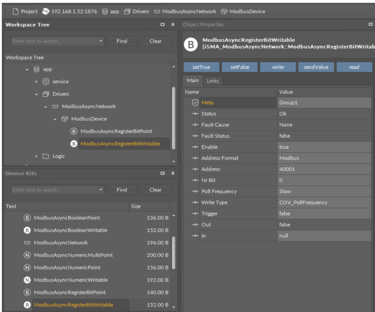
Figure 11. ModbusAsyncRegisterBitWritable component
